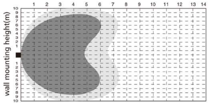
((( ))) Wall Mounting pattern (Unit: m)
