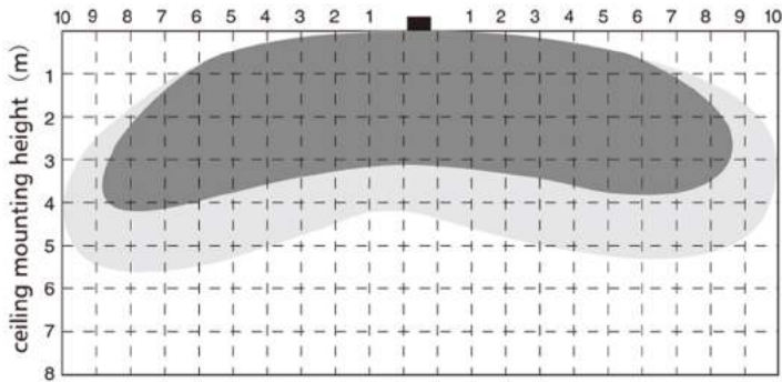
((( ))) Ceiling Mounting pattern (Unit: m)
